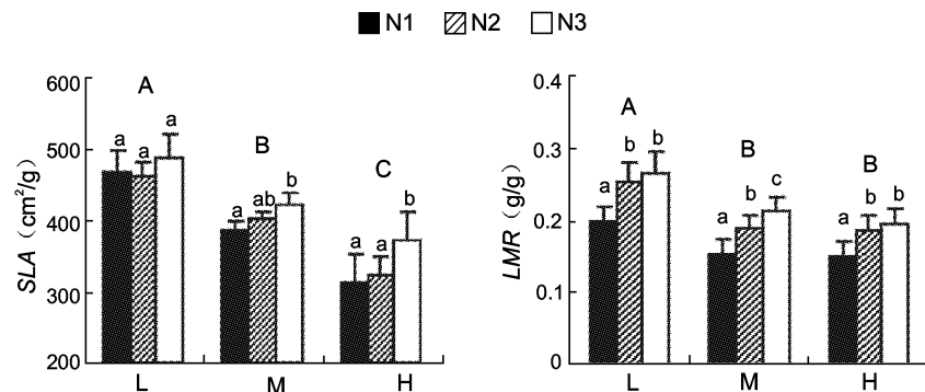
图 3 不同光强和施氮处理下的比叶面积和叶生物量比 Fig. 3 Specific leaf area and Leaf mass ratio under different light intensity and nitrogen level
